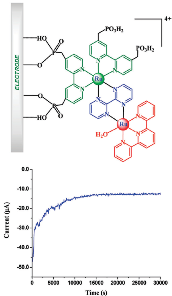
Fig. 121 Electrolysis of [(4,4'-(\text{HO})_2\text{P}(\text{O})\text{CH}_2)_2\text{bpy}]_2\text{Ru}(\text{bpm})-\text{Ru}(\text{tpy})(\text{OH})_2]^{4+} on FTO at 1.8 V in 1.0 M \text{HClO}_4 : turnovers > 8900 ; rate) 0.3 \text{ s}^{-1} ; current density \approx 6.7 \mu\text{A cm}^{-2} ; \Gamma \approx 7 \times 10^{-11} \text{ mol cm}^{-2} ; (A) 1.95 \text{ cm}^2 . For [(4,4'-(\text{HO})_2\text{P}(\text{O})\text{CH}_2)_2\text{bpy}]_2\text{Ru}^{\text{II}}(\text{bpm})\text{Ru}^{\text{II}}(\text{Mebimpy})(\text{OH})_2]^{4+} on FTO at 1.8 V in 1.0 M \text{HClO}_4 : turnovers > 28000 ; rate) 0.6 \text{ s}^{-1} ; current density \approx 14 \mu\text{A cm}^{-2} ; \Gamma \approx 7 \times 10^{-11} \text{ mol cm}^{-2} ; (A) 1.95 \text{ cm}^2 . Reprinted with permission from ref. 1495 Copyright Wiley 2009. American Chemical Society.
