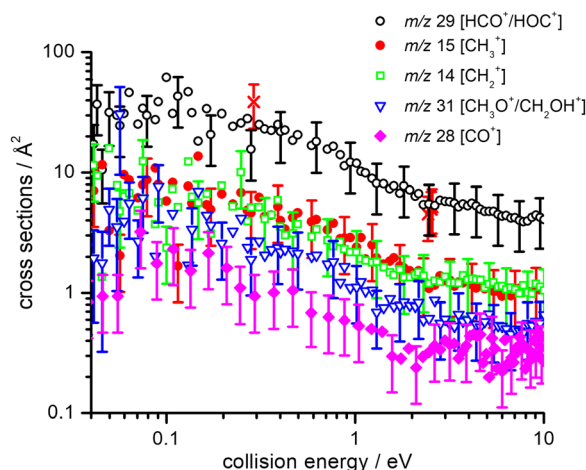
Fig. 1 Absolute CSs (in \text{\AA}^2 ) for the production of \text{HCO}^{*+}/\text{HOC}^{*+} (black open circles), \text{CH}_3^{*+} (red filled circles), \text{CH}_2^{*+} (green open squares), \text{CH}_3\text{O}^{*+}/\text{CH}_2\text{OH}^{*+} (blue open triangles) and \text{CO}^{*+} (magenta filled diamonds) ionic products as a function of the collision energy ( E_{\text{CM}} ), from the title reaction.
