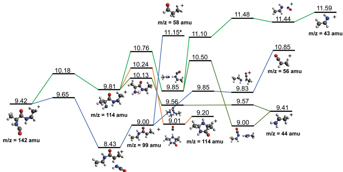
Fig. 6 Two different paths after the most probable ring opening CO-/CHCH 3 (see Fig. 5a). The green path follows the direct formation of CO and its evolution while the lower blue path follows the evolution after the release of HNCO. Relative energies are given in eV, referred to the neutral molecule and were obtained at a B3LYP/6-311++G(d,p) level of theory. The blue path leading to fragment 58 + , indicated with a *, is presented and further discussed in Section S4 in the ESI.†
