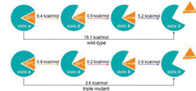
Fig. 8 Two series of free energy simulations for protein structural changes from holo closed state to apo open state. Orange arrows – Free energies of holo protein opening from metadynamics. Red arrows – \Delta\Delta G_{\text{binding}} from alchemical simulations. Blue arrows – GLYCAM glucose unbinding energies from funnel metadynamics.
