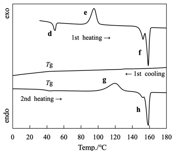
Fig. 6 DSC curves of OC6-salmpn left in glass state for 1 year; heating and cooling rate: 5 °C min -1 .
