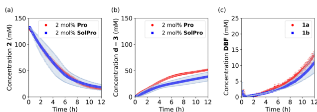
Fig. 1 Kinetic experiments examining individual reactions involved in cross-catalytic system at 25^\circ\text{C} in acetone- d_6 as the solvent. (a) and (b) Mannich reaction between acetone- d_6 and 2 (133 mM) catalysed by 2 mol% of Pro (red circles) and 2 mol% of SolPro (blue squares); (c) the deprotection of 1a (red circles) and 1b (blue squares) (133 mM) with 1 equiv. of d-3 . 24
