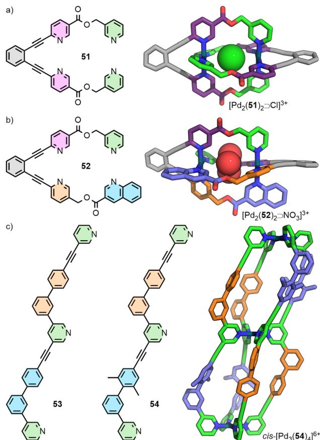
Fig. 10 Covalent trans -tethering of (a) identical ditopic ligand fragments enables access to Pd_2L_2 cages with a pseudo- trans - Pd_2L_4 cavity (SCXRD structure), and (b) different ditopic units generates a pseudo- Pd_2L_2L'_2 cavity of C_2 symmetry (SCXRD structure). (c) Unsymmetrical tritopic ligands 53 and 54 assemble to give trinuclear cis - Pd_3L_4 cages (PM6 model) where each cavity can be described as a pseudo- Pd_2L_2L'_2 environment.
