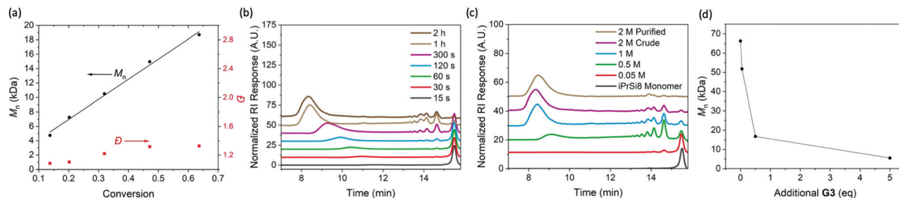
Fig. 1 Characterization of the polymerization and depolymerization of 1PrSi8 . (A). Plot of M_n and D vs monomer conversion, obtained by a combination of SEC and ^1\text{H} NMR analysis. (B) SEC traces (normalized RI) of poly(1PrSi8) quenched at different reaction times (correlated to Table 1, entries 6–12). (C) SEC traces of poly(1PrSi8) prepared at increasing monomer concentration in dioxane (correlated to Table 2, entries 1–5). (D) Polymer size (obtained by SEC) of homopolymer prepared from 500 mM 1PrSi8 (Table 2, entry 2) as it is exposed to increasing amounts of additional G3 .
