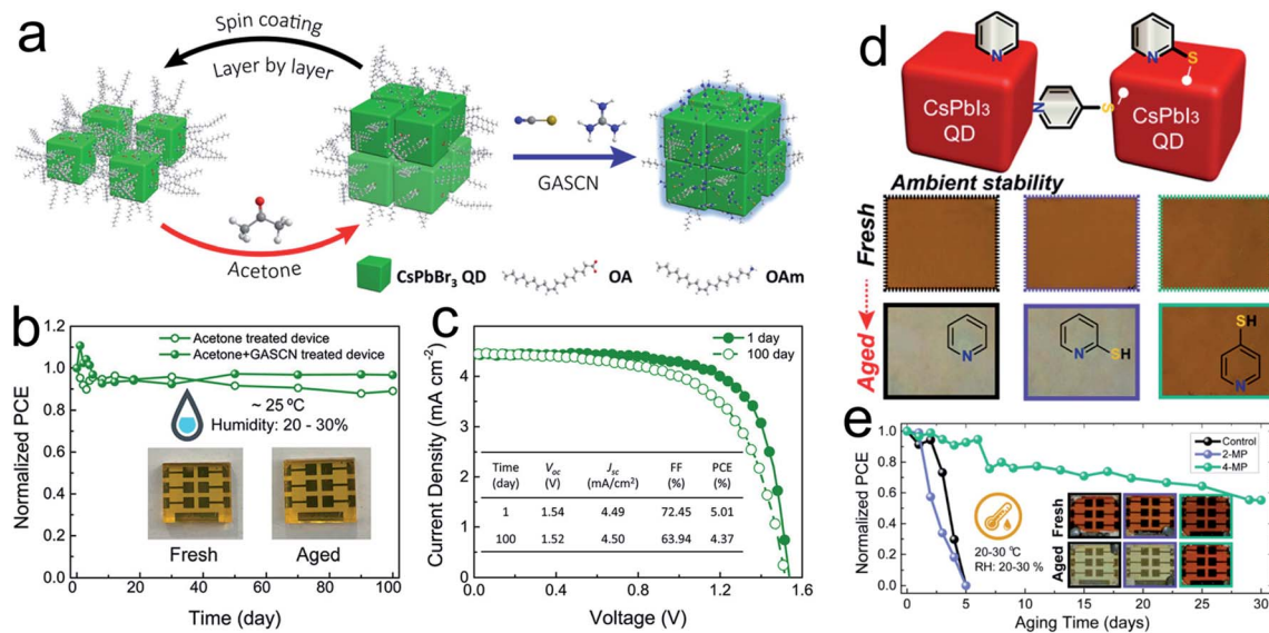
Fig. 17 QD treatment for stability. (a) Schematic illustration of \text{CsPbBr}_3 QD film deposition and solid-state post-treatment. (b) Long-term stability characterization of an optimal \text{CsPbBr}_3 QD SC compared with the acetone-treated device. Inset images show the photographs of the corresponding optimal devices after storage for different days. (c) J - V curves of the corresponding optimal device after storage for different days. Adapted with permission from ref. 192 Copyright 2020, American Chemical Society. (d) QD film stability of \text{CsPbI}_3 QD based on MeOAc treatment (control) and 2-MP and 4-MP post-treatment. (e) Ambient stability of \text{CsPbI}_3 QD SC devices based on MeOAc treatment (control) and 2-MP and 4-MP post-treatment under an RH of 20–30%. Adapted with permission from ref. 177 Copyright 2020, American Chemical Society.
