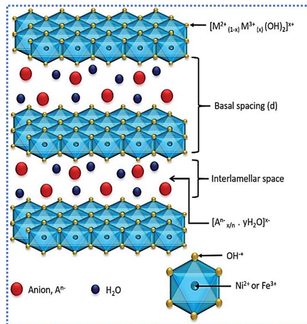
Fig. 1 The structure of the NiFe-layered double hydroxide.
