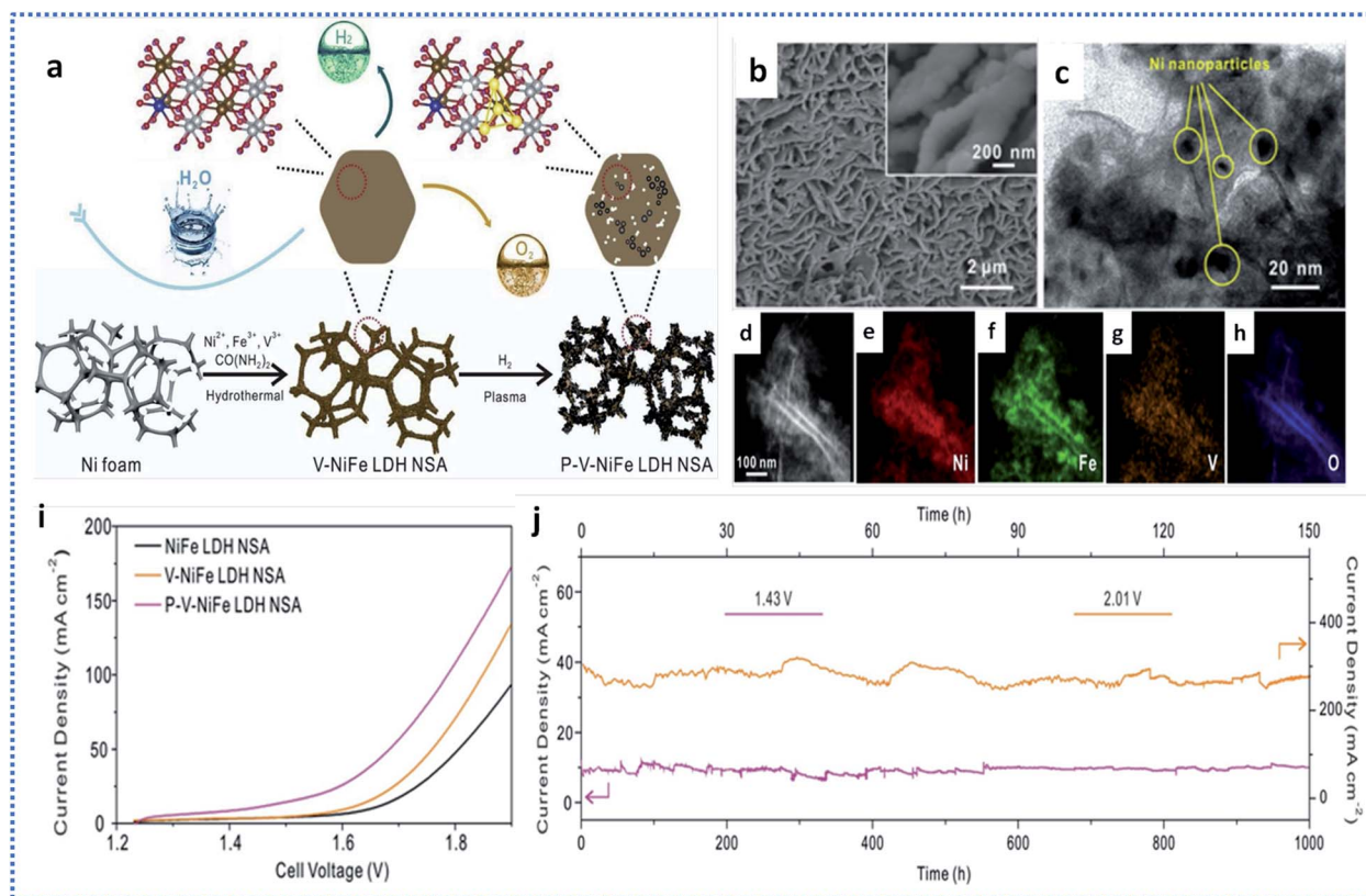
Fig. 15 (a) Schematic illustration of the fabrication process of P-V-NiFe LDH NSA. (b) SEM image. (c) TEM image. (d-h) HAADF-STEM and corresponding elemental mapping images of P-V-NiFe LDH NSA. (i) Overall water splitting performance of NiFe LDH, V-NiFe LDH NSA, and P-V-NiFe LDH NSA. (j) CA tests at 1.43 V for P-V-NiFe NSA. Reproduced with permission. 227 Copyright 2020, Elsevier.
