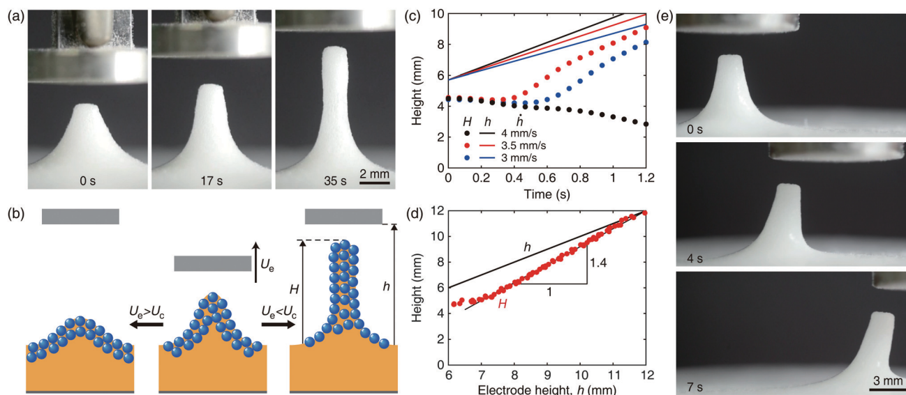
Fig. 3 Morphology control of the particle raft. (a) Images of a raft tower pulled vertically following the electrode that ascends from h = 6.4 to 10 mm at a speed of 0.1 \text{ mm s}^{-1} . (b) Schematics of a particle raft that either collapses or grows depending on whether the electrode ascends at a speed higher or lower than the critical speed U_c . (c) Temporal evolution of the hill height (solid lines), which starts from H = 4.5 \text{ mm} with h = 5.7 \text{ mm} , for different ascent speeds of the electrode, U_e = 3, 3.5 , and 4 \text{ mm s}^{-1} . The particle raft grows upward following the electrode when the ascent speed is 3 and 3.5 \text{ mm s}^{-1} , but it collapses when U_e = 4 \text{ mm s}^{-1} . The dotted lines indicate the elevation of the electrodes, h . (d) The change of the raft height H as the electrode rises at U_e = 0.1 \text{ mm s}^{-1} . (e) Horizontal translation of a tower following the electrode horizontally moving at a speed of 2 \text{ mm s}^{-1} . In (a) and (c)–(e), the electric potential \phi is 10 kV.
