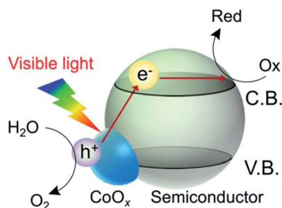
Scheme 1 Water oxidation driven by charge transfer from a loaded Co species ( e.g. , CoO x ) to a semiconductor support. Even though the bandgap photoexcitation of the semiconductor from the valence band (V.B.) to the conduction band (C.B.) under visible light is not possible because of the large bandgap of the semiconductor, interfacial charge transfer from Co to the semiconductor may occur under visible light.
