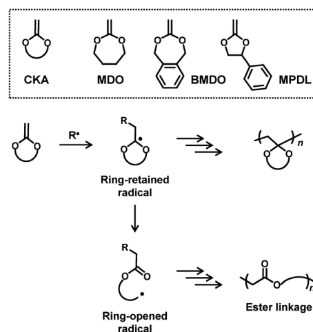
Scheme 1 CKA monomers and their possible polymerization mechanisms.
