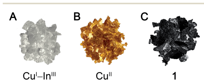
Fig. 1 Photographs of crystals of (A) the colorless double perovskite, (PEA) 4 Cu I In III Cl 8 , (B) the yellow single perovskite, (PCA) 2 Cu II Cl 4 , and (C) the black perovskite, (BA) 4 [Cu II (Cu I In III ) 0.5 Cl 8 ] ( 1 BA ), featuring a 1 : 1 blend of the inorganic lattices in A and B. The black color arises from Cu +2+ mixed valency. PEA = phenethylammonium, PCA = p -chloroanilinium, and BA = butylammonium.
