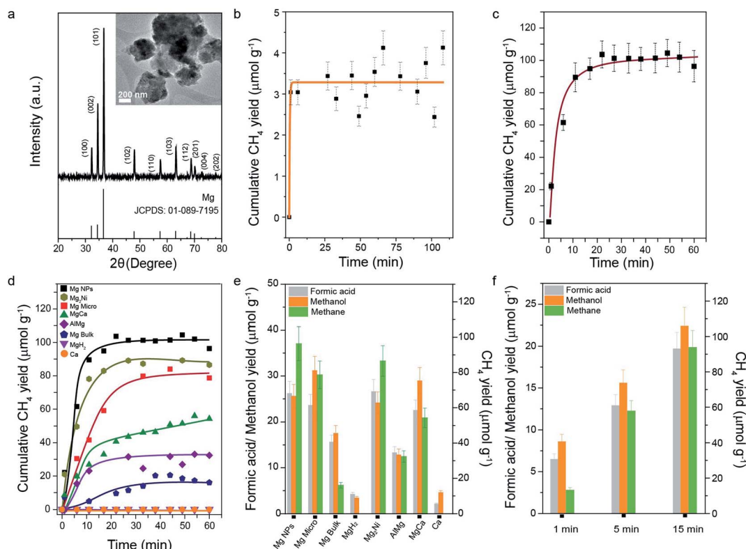
Fig. 1 (a) PXRD patterns (TEM image in the inset) of Mg NPs along with the standard XRD pattern of Mg (JCPDS no. 01-089-7195); cumulative methane yield with reaction time for CO 2 reduction using Mg NPs using (b) CO 2 directly from the air and (c) 99.99% CO 2 ; (d) comparison of yields of various metals and Mg–metal alloys (99.99% CO 2 ); (e) methanol, formic acid, and methane yields after 1 h, for CO 2 (99.99%) reduction on Mg NPs, micro powder and bulk Mg, Mg–metal alloys, MgH 2 and Ca metal; (f) methane, methanol, and formic acid yield quantified after 1, 5, and 15 min, for reduction of CO 2 using Mg NPs. All reactions were carried out in water at room temperature and atmospheric pressure. Error bars are omitted in (d) for clarity and were less than 10%. The selectivity for carbon-containing products such as methane, methanol and formic acid is given in Fig. S2.†
