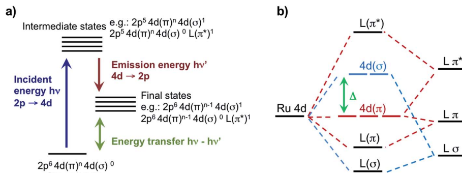
Fig. 1 (a) Illustration of the 2p4d RIXS experiment. The process starts with the creation of a 2p-hole by monochromatic X-rays with incident energy at the resonances of the L-edge XAS spectrum. Following creation of a 2p-hole, 4d \rightarrow 2p emission lines are collected. The energy difference of the incident and emitted X-rays defines an energy transfer that results from valence excitations in the final state. (b) Illustration of the molecular orbitals with mixed Ru 4d and ligand (L) character in the ligand field picture. The 4d( \pi ) and the 4d( \sigma ) orbitals, which in octahedral symmetry corresponds respectively to the t_{2g} and e_g orbitals, are separated by the ligand field splitting energy ( \Delta ).
