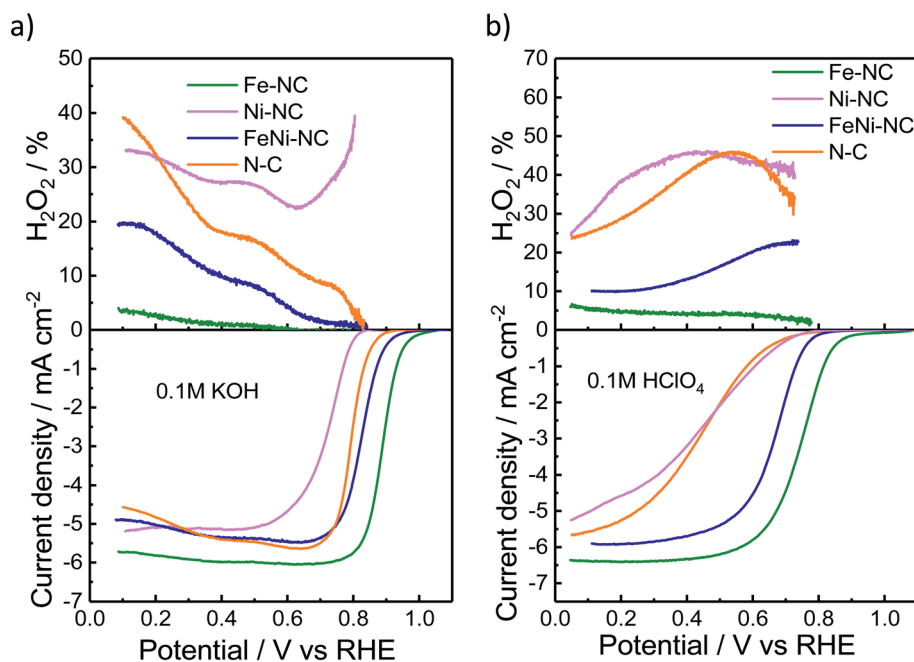
Fig. 2 Electrochemical activity evaluation. \text{H}_2\text{O}_2 percentage and disk current density from rotating-ring disk electrode (RRDE) experiments of MNC catalysts at 1600 rpm in oxygen-saturated (a) alkaline and (b) acidic electrolytes.
