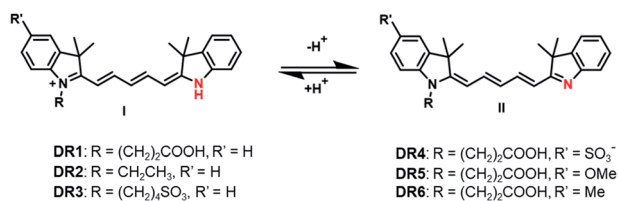
Scheme 1 The chemical structures of the unsymmetrical pentamethine cyanines upon protonation and deprotonation.
