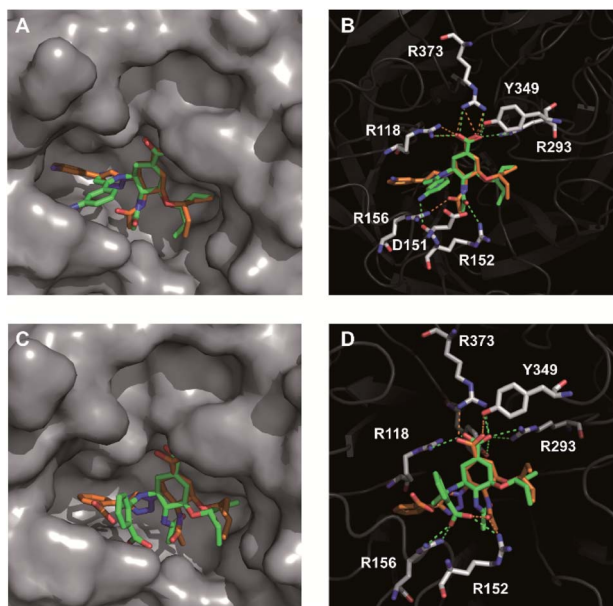
Fig. 3 Comparison of the binding modes and interactions of 5'-substituted 1,2,3-triazolylated OSC derivatives (green) and their 4'-isomers (orange) with N5 neuraminidase. (A and B) Overlay of N5-1j with N5-2j; (C and D) Overlay of N5-1h and N5-2h. Polar interactions are represented by dashed lines (green for the 2 series and orange for the 1 series). Other interactions are not shown. The residues involved in direct hydrogen bonds with the ligand are represented with sticks. The oxygen and nitrogen atoms of the compounds are colored red and blue, respectively.
