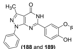
Fig. 61 Chemical structures of selected pyrazolopyrimidines (188 and 189).
