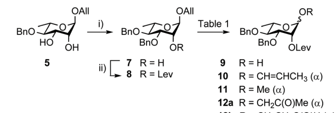
Scheme 2 Synthesis of hemiacetal 9 from diol 5 . (i) BnBr, Fe(dibm) 3 or Fe(dipm) 3 (5 mol%), K 2 CO 3 , MeCN, 80 °C, 92%; (ii) LevOH, EDC, DMAP, DCM, 90%. dibm: diisobutylmethane; dipm: dipivaloylmethane; LevOH: levulinic acid.
