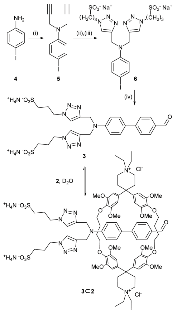
Scheme 2 Synthesis of 3 and pseudorotaxane formation with 2 in D_2O . (i) Propargyl bromide (30 wt% in toluene), K_2CO_3 , ACN, 60 °C, 3 d, 66%; (ii) NaN_3 , 1,3-propanedithiol, DMF/ H_2O (2:1), rt, 1 h; (iii) TBTA, Cu (CH_3CN)_4PF_6 , sodium ascorbate, 5 , rt, 22 h, 45%; (iv) 4-formylphenylboronic acid, K_3PO_4 , Pd(OAc)_2 , H_2O , reflux, 1 h, 78%.
