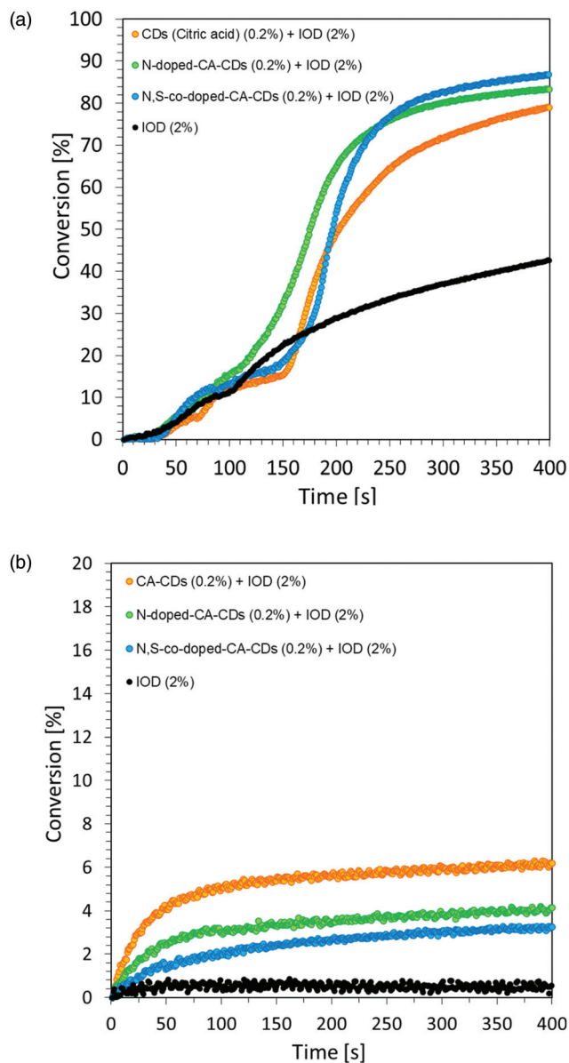
Fig. 7 Cationic photopolymerization profiles (vinyl function conversion vs. irradiation time) initiated by a bimolecular photoinitiating system based on IOD (2.0 wt%) and CDs (0.2 wt%) (a) under irradiation at 365 nm and (b) under irradiation at 405 nm.
