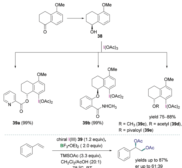
Scheme 16 Synthesis of the tetraol-based chiral trivalent iodine compounds (top); stereoselective diacetoxylation using trivalent iodine compounds (bottom).
