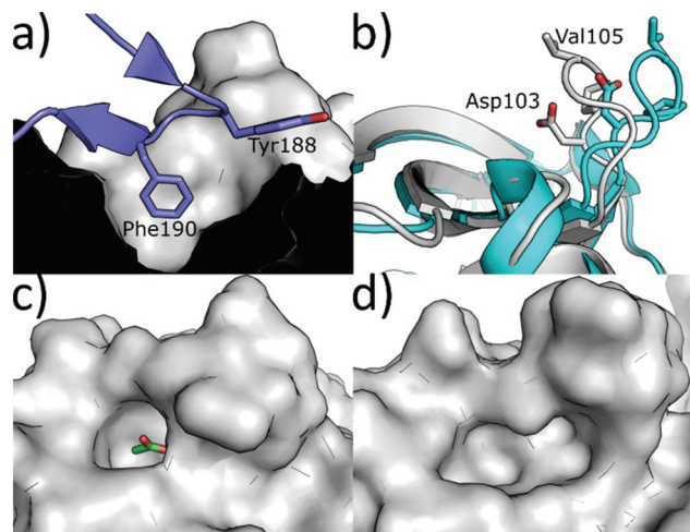
Fig. 8 (a) CK2β interface loop (purple) binding in the CK2α interface site (grey) (PDB: 4MD7). (b) Flexibility of the interface site. Open/peptide bound structure in cyan (PDB: 6Q4Q), closed/small molecule bound structure in grey (PDB: 5CU6). (c) Surface of the closed/small molecule bound structure (PDB: 5CU6) and (d) surface of the open/peptide bound structure (PDB: 6Q4Q). Ligand is shown in green and the surface in grey.
