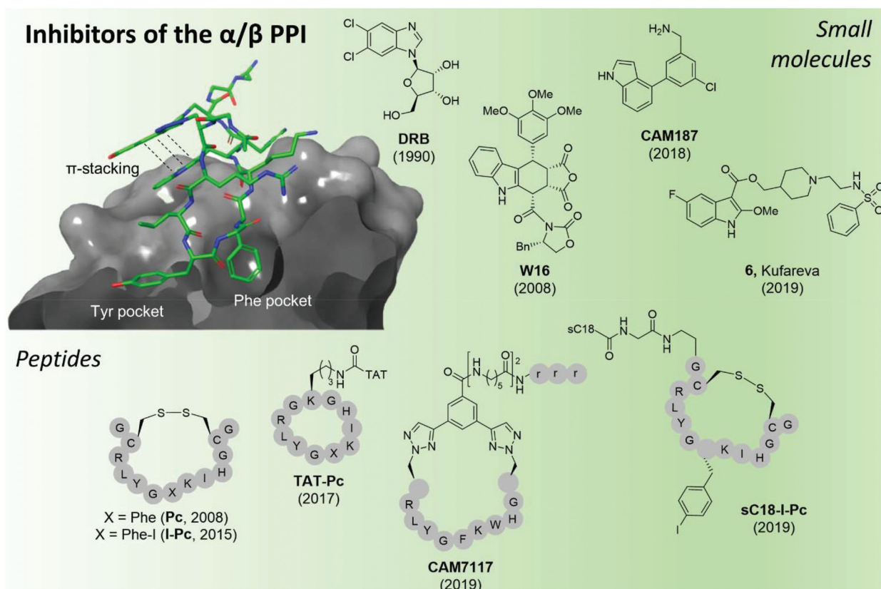
Fig. 9 CK2 inhibitors reported in chronological order and acting at the protein interface between the catalytic and regulatory subunit with the co-crystal structure of CK2α and CAM7117 shown on the left (PDB: 6Q4Q). The hydrophobic Tyr and Phe pockets key to binding are highlighted, alongside the \pi - \pi stacking interactions of the ligand. sC18 = \text{H}_2\text{N} -GLRKRLRKFRNKIEK- \text{NH}_2 , 93 TAT = GRKKRRQRRRPPQ. 96 Compounds have been labelled as in the related papers. r = D-Arg.
