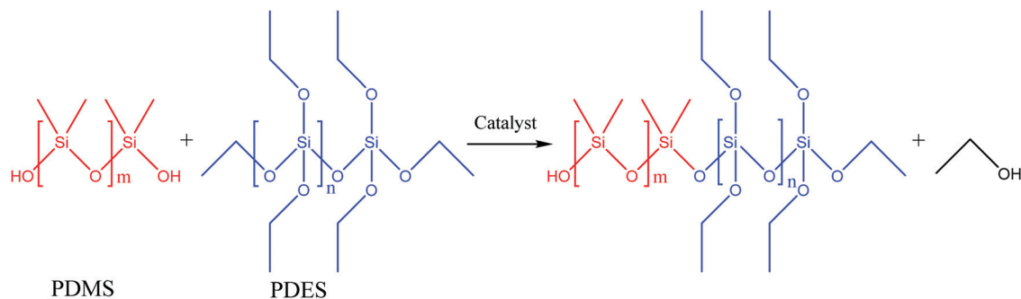
Fig. 19 Schematic illustration of polycondensation between HOPDMS and PDES [reproduced from ref. 3 with permission from Elsevier].
