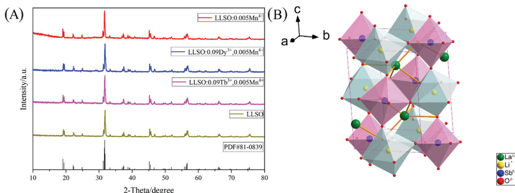
Fig. 1 (A) XRD patterns of \text{LLSO}:\text{0.005Mn}^{4+} , \text{LLSO}:\text{0.09Tb}^{3+},\text{0.005Mn}^{4+} , \text{LLSO}:\text{0.09Dy}^{3+},\text{0.005Mn}^{4+} and LLSO host. (B) Crystal structure schematic diagram of \text{La}_2\text{LiSbO}_6 .
