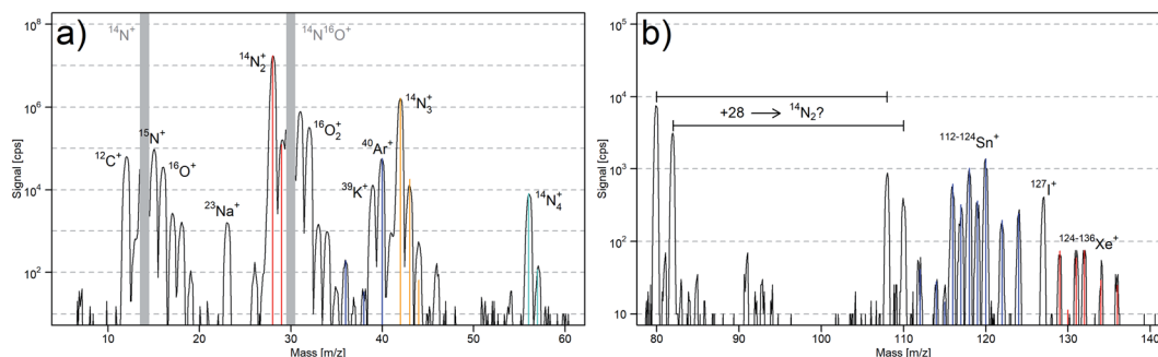
Fig. 3 Dry (N 2 -ICP)-MS gas blank spectra. (a) Isotopic abundance of 14 N 2 – 14 N 15 N (red), Ar (blue), 14 N 3 – 14 N 2 15 N – 14 N 15 N 2 (orange), and 14 N 4 – 14 N 3 15 N (light blue). (b) Isotopic abundance of Sn (blue), Xe (red) and signals at m/z 80, 82, 108, and 110 not assigned yet.
