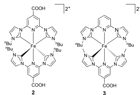
Fig. 2 Structures of the sensitizers 2 and 3 . Both complexes were isolated and used in DSCs as the [PF 6 ] - salts.
