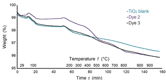
Fig. 7 TGA curves for blank TiO 2 (green), TiO 2 sensitized with dye 2 (purple) and TiO 2 sensitized with dye 3 (grey).
