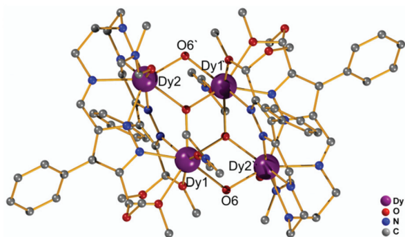
Fig. 1 Molecular structure of the cation of \text{Dy}_4 . Hydrogen atoms and counterions have been omitted for clarity.
