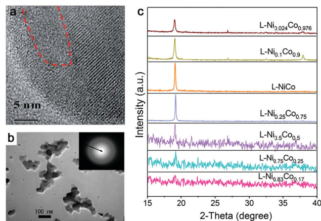
Fig. 4 Amorphous metal oxides by laser ablation in water. (a) HRTEM of FeO x NPs after laser irradiation showing some amorphous domains. Reproduced with permission from ref. 150. (b) TEM image of amorphous Pt NPs by LAL at a wavelength of 355 nm and a laser fluence of 4 J cm -2 . Reproduced with permission from ref. 155. (c) XRD patterns of products with different proportions of Co and Ni by laser ablation in 1 M KOH. Reproduced with permission from ref. 159.
