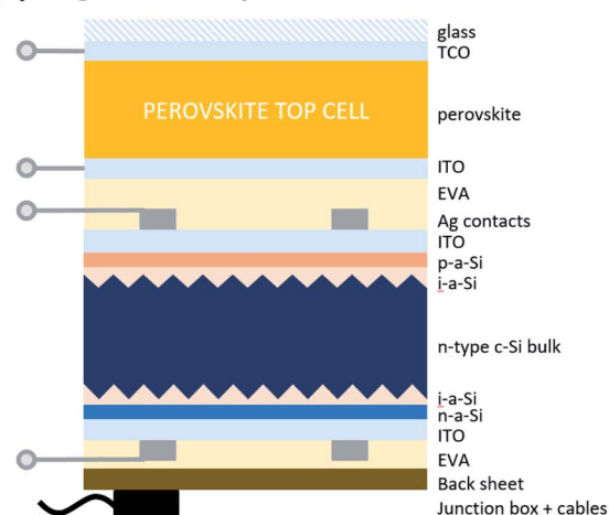
Fig. 1 Schematic of the two silicon single-junction modules and the two 4T tandems. These schematics indicate the full stack used for the module manufacturing.
