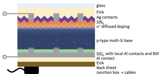
(a) 'Low-cost' silicon SJ cell
