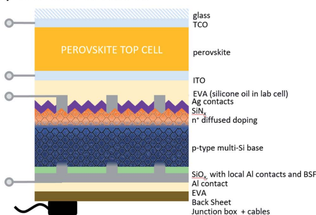
(c) 'Low-cost' 4T tandem
