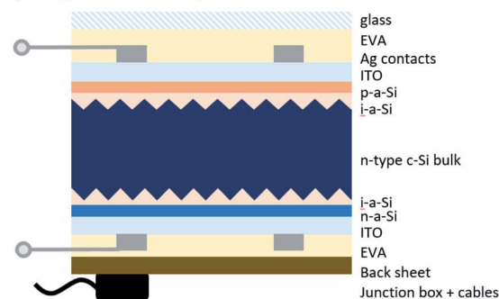
(b) 'High-efficiency' silicon SJ cell
