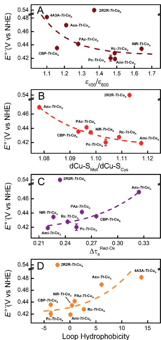
Fig. 5 Reduction potentials of the Tt -Cu A chimeras as function of (A) the experimental \epsilon_{450}/\epsilon_{600} ratio, (B) the calculated dCu-S_{Met}/dCu-S_{Cys} ratio, (C) the calculated \Delta\tau_4 = \tau_4 (red) - \tau_4 (ox) parameter and (D) the hydrophobicity of the ligand loop. Dashed lines are included to guide the eye. Error bars represent the standard deviation of no less than 3 independent measures.
