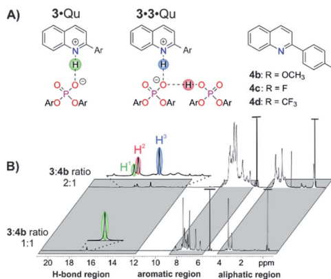
Fig. 7 (A) Schematic structures of the 3 ·Qu and 3 · 3 ·Qu complexes and substituents of quinolines 4b–d . (B) Spectral resolution of the ^1\text{H} spectra of complexes of 3 and 4b at a 1 : 1 or 2 : 1 stoichiometry at 200 K and 600 MHz in \text{CD}_2\text{Cl}_2 . In the 1 : 1 system, only one H-bond is detected, presumably of the 3 · 4b complex. For the 2 : 1 system, three major H-bonds are observed at 16.76 (H1), 16.51 (H2) and 15.27 ppm (H3), most likely of the 3 · 4b (H1) and 3 · 3 · 4b (H2 and H3) complex.
