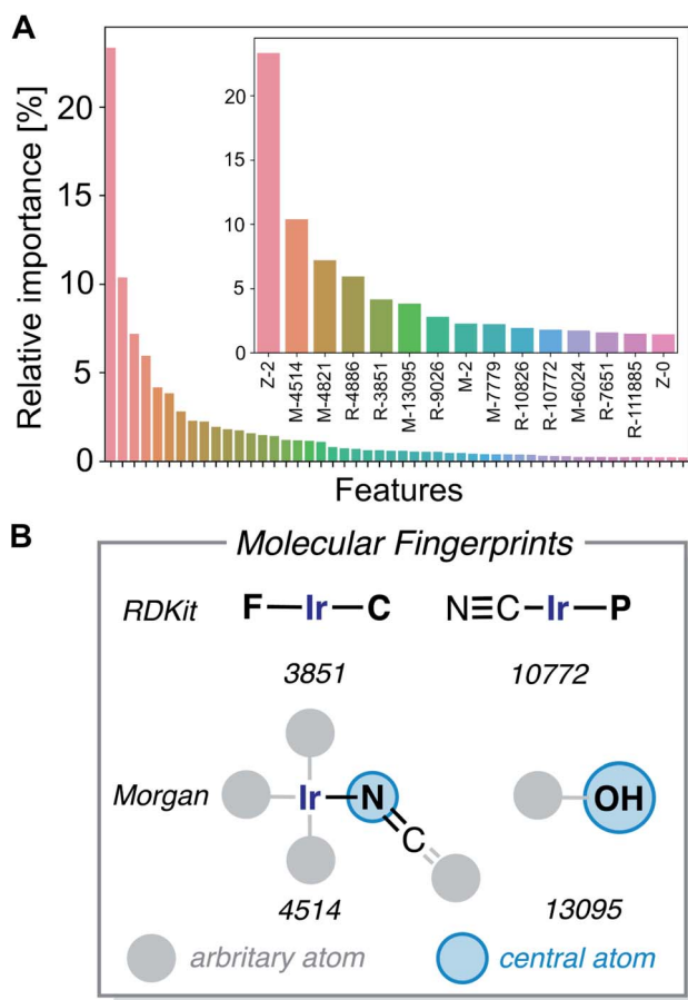
Fig. 9 (A) Most important features for the performance of the gradient boosting regression model; (B) Illustration of four of the most important molecular subgraphs corresponding to features RDKit 3851, 10772, and Morgan 4514, 13095. Morgan fingerprints are circular fingerprints centered at a given atom (marked in blue).
