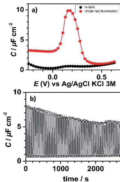
Fig. 3 (a) Capacitance–potential curves of SAM-1-Rad-Si measured at 50 \text{ Hz} in the dark and under red light illumination. (b) Capacitance–time profile at 50 \text{ Hz} measured at 0.18 \text{ V} during dark (OFF state, 30 \text{ s} )/illumination (ON state, 30 \text{ s} ) switching cycles. Electrolytic solution: \text{CH}_3\text{CN} + 0.1 \text{ M Bu}_4\text{NClO}_4 .
