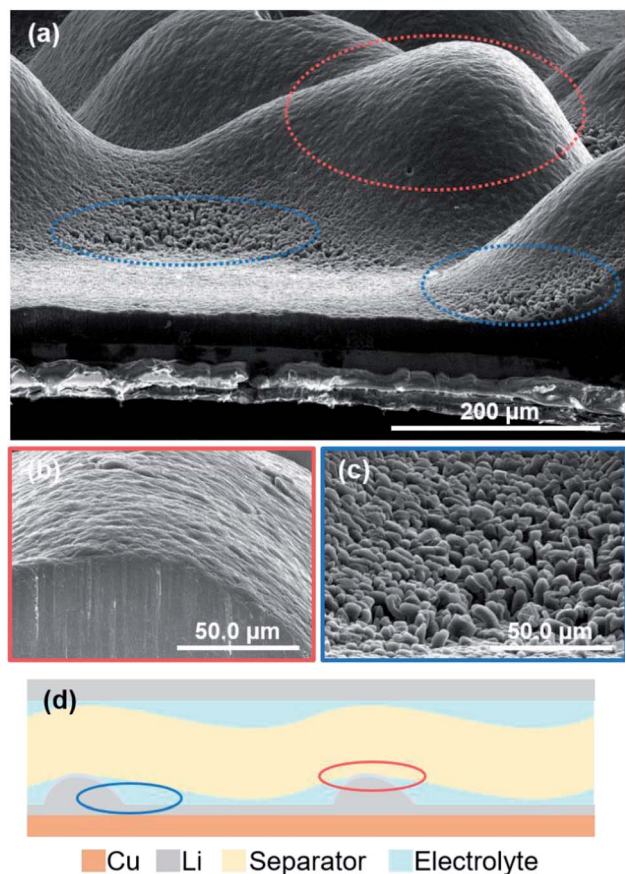
Fig. 9 (a) Cross-sectional SEM images of the electrodeposited lithium metal after plating on the copper substrate at 15 \text{ mA h cm}^{-2} under a pressure of 1.39 MPa. Expanded images at (b) the convex portion and (c) the concave portion. (d) Schematic diagram of the morphology of electrodeposited lithium in contact with a separator with poor flatness.
