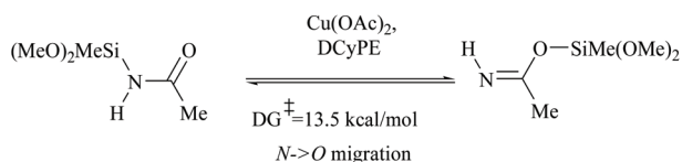
Scheme 30 DFT calculations: Cu catalyzed interconversion of N -silyl and O -silyl imidate forms.
