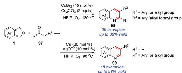
Scheme 38 Cascade annulation reaction of anthranils with 1,3-diketones/aldehydes.
