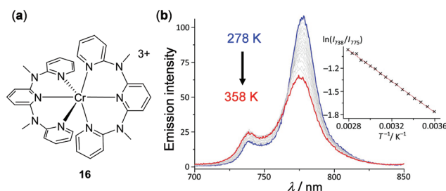
Fig. 15 (a) Molecular structure of Cr(III) complex 16 with \text{BF}_4^- counter anions. (b) Temperature-dependent emission spectra of 16 in air-saturated \text{H}_2\text{O} from 278 to 358 K. Inset: The related Boltzmann fitting plots of \ln(I_{738}/I_{775}) vs. T^{-1} . The emission changes are reversible. Reprinted with permission from ref. 104. Copyright 2017 Wiley-VCH.
