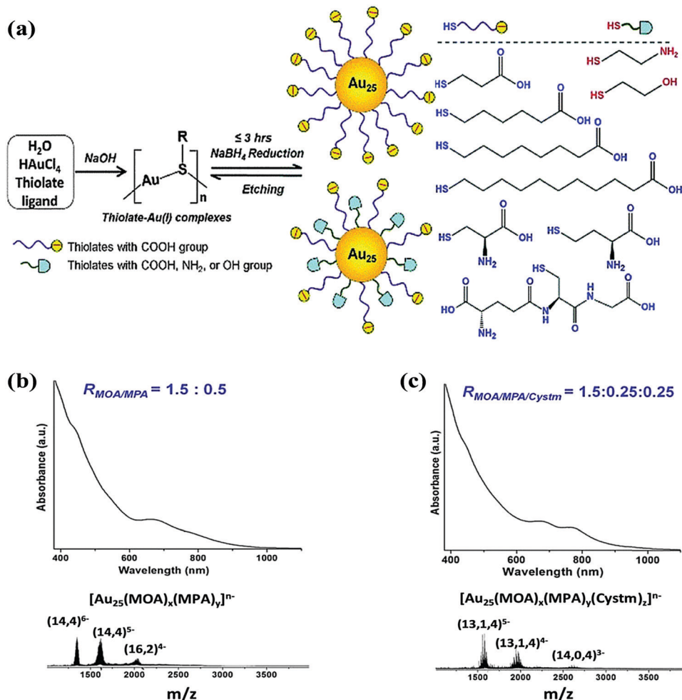
Fig. 2 (a) Schematic illustration of NaOH-mediated NaBH 4 -reduction protocol for the synthesis of thermodynamically stable thiolate-protected Au 25 NCs. (b) UV-Vis absorption (top) and ESI mass (bottom) spectra of the as-synthesized bi-thiolate-protected Au 25 NCs. (c) UV-Vis absorption (top) and ESI mass (bottom) spectra of the as-synthesized tri-thiolate-protected Au 25 NCs (here MOA denotes 8-mercaptooctanoic acid; MPA denotes 3-mercaptopropionic acid; and Cystm denotes cysteamine). Reproduced with permission. 105 Copyright 2014, Wiley-VCH.
