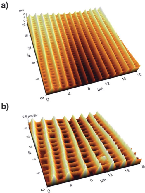
Fig. 3 (a) The topography of an area ( 10\text{ }\mu\text{m} \times 10\text{ }\mu\text{m} ) of a single scale of A. urticae imaged by atomic force microscopy. There are about 13 ridges per 10\text{ }\mu\text{m} . (b) The topography of I. leuconoe shows the same type of structure but the overall size of the ridges is scaled. The distance and height of the ridges are nearly twice as much compared to A. urticae (approx. 7 ridges per 10\text{ }\mu\text{m} ).
