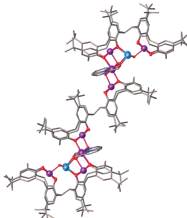
Fig. 2 Symmetry-expanded structure of 6 showing the central bridging syn -L octa-anion. Colour code C – grey, O – red, N – royal blue, Mn II – pale blue, Mn III – purple. Hydrogen atoms, ligated solvent molecules and co-crystallised solvent/anions omitted for clarity.
