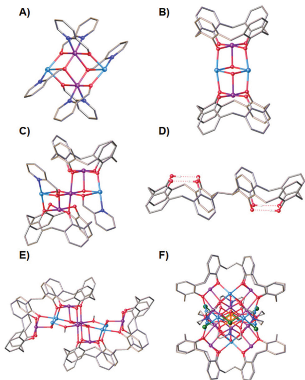
Fig. 1 Single crystal X-ray structures of 1 (A), 2 (B), 3 (C), H 8 L1 (D), 4 (E) and 5 (F). Colour code C – grey, O – red, N – royal blue, Mn II – pale blue, Mn III – purple, Cl – green, H – white. Hydrogen atoms (except those involved in lower-rim H-bonding in D), t Bu groups, ligated solvent molecules and co-crystallised solvent/anions omitted for clarity.
