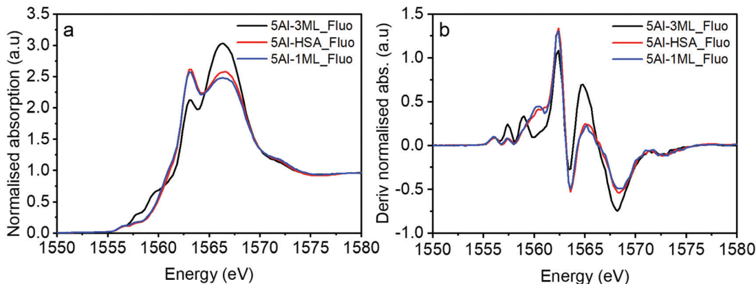
Fig. 8 (a) XAS spectra of the 5% Al haematite sample coated with Mo and (b) its derivative.
