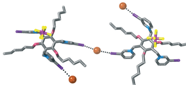
Fig. 9 Structure of 4-Br 1.5 ·(PF 6 ) 1.5 . Hydrogen atoms omitted for clarity.
