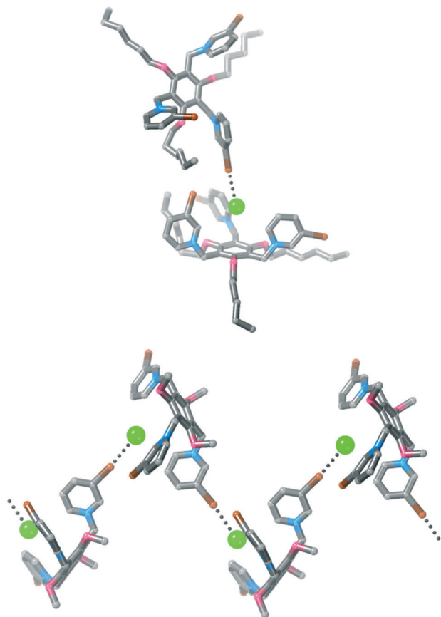
Fig. 7 Two views of the structure of 3-Cl 3 showing the 1D polymeric structure. Hydrogen atoms, disorder, solvent molecules and some chloride anions have been omitted for clarity.
