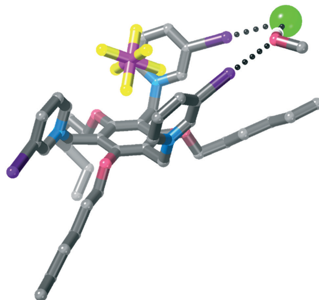
Fig. 8 Structure of 4-Cl·(PF 6 ) 2 . Hydrogen atoms and one of the hexafluorophosphate anions are omitted for clarity.
