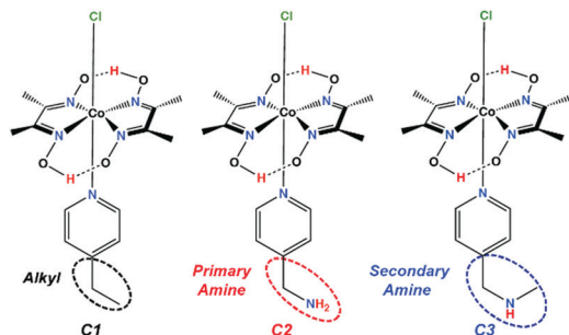
Scheme 1 Schematic structures of the complexes C1–C3 . The dotted ellipses highlight the outer coordination sphere (OCS) functionalities around the cobaloxime core.
