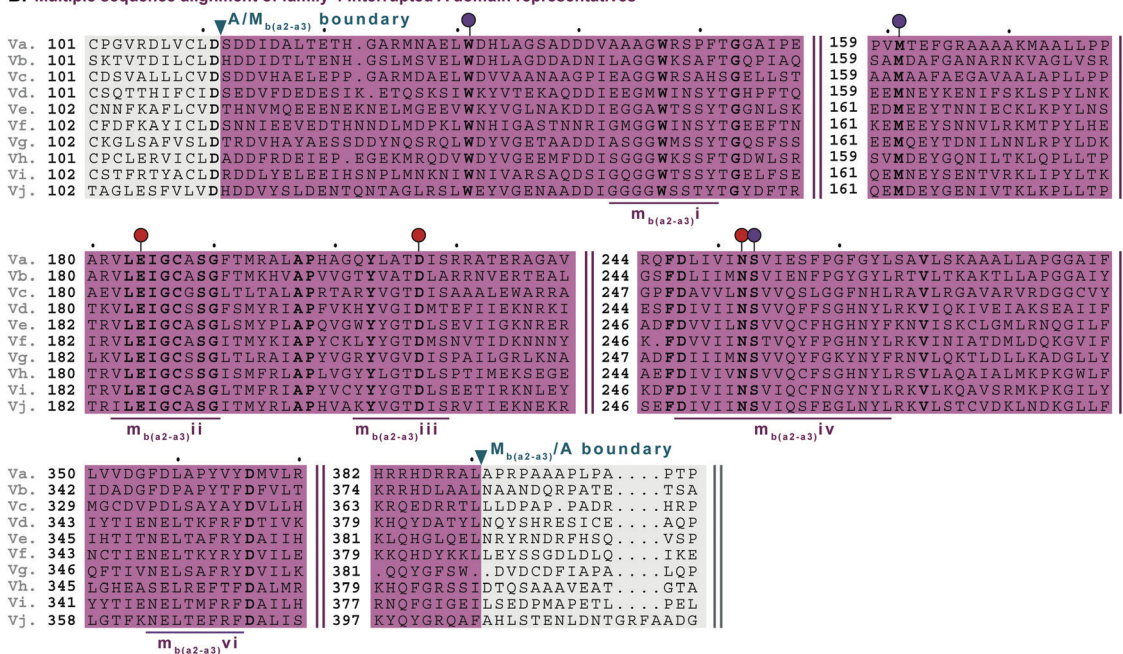
Fig. 6 Multiple sequence alignments of (A) family 1 (type I M domain) interrupted A domain representatives as noted in Fig. S1 (ESI†), and (B) family 4 (type V M domain) interrupted A domain representatives as noted in Fig. S5 (ESI†). Types I and V M domains are highlighted in light purple and light pink, respectively. The A domain is highlighted in light grey. The red and dark purple balloons in panel A correspond to residues involved in SAM and amino acid bound Ppant arm binding, respectively, according to the structure of \text{TiO}_2(\text{Ag}_2\text{M}_2\text{Ag})_4 . 14 The identical corresponding residues in type V M domain are also indicated in the same way. The conserved M domain motifs for types I and V M domains are underlined in dark purple and dark pink, respectively. The boundaries between the domains are indicated by a triangle. Breaks in the sequences are indicated by two parallel bars. The full sequence alignments and accession numbers are presented in Fig. S13 and S16 (ESI†).
