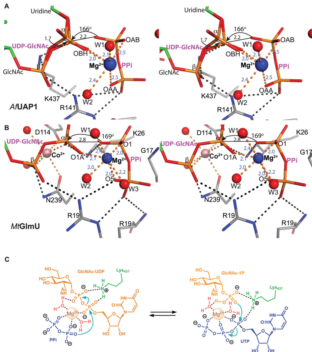
Fig. 5 Magnesium coordination and AfUAP1 mechanism. (A) Magnesium coordination in the AfUAP1-UDP-GlcNAc-PPi-Mg 2+ complex active site. A view of the active site of the AfUAP1-UDP-GlcNAc-PPi-Mg 2+ and MtGlmU-UDP-GlcNAc-PPi-Mg 2+ -Co 2+ complexes. The attack distance for pyrophosphorolysis is 2.2 and 2.8 Å and the attack angle is 166° and 169° for UAP1 and GlmU, respectively. The distance between the α-phosphates in both UDP-GlcNAc adopting the dual conformation is 1.7 Å. The Mg 2+ is tetragonal bipyramidally coordinated (albeit with a disordered 6th ligand in AfUAP1) as suggested by coordination distances and angles. (B) Magnesium coordination in the MtGlmU-UDP-GlcNAc-PPi-Mg 2+ -Co 2+ complex active site. (C) Schematic diagram of the proposed forward and reverse reaction mechanisms. The left panel indicates chemical bond formation/cleavage (cyan arrows) in the AfUAP1-PPi-UDP-GlcNAc ternary complex shown in Fig. 5A leading to the formation of GlcNAc-1P and UTP. The right panel using the same ternary complex structure as a template indicates chemical bond formation/cleavage in the reverse reaction leading to the formation of UDP-GlcNAc and PPi from GlcNAc-1P and UTP is proposed.
