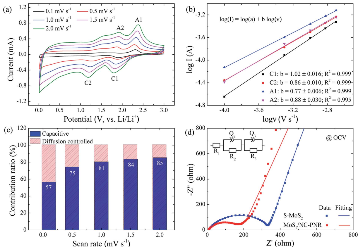
Fig. 8 Kinetic analysis of MoS 2 /NC-PNR as LIB anode: (a) CV curves at different scan rate; (b) current response versus scan rate (log I vs. log v) plots at each redox peak; (c) capacitive and diffusion controlled contributions to the electrochemical processes at corresponding scan rate; the number labels the percentile capacitive contributions; (d) Nyquist plots and the fitting curves of MoS 2 /NC-PNR and S-MoS 2 electrodes. The inset shows the equivalent circuit.
