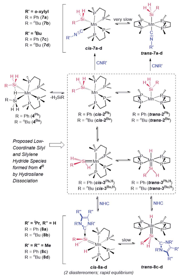
Scheme 5 Trapping of putative silyl (2 R ) and silylene hydride (3 R,H ) intermediates: synthesis of silyl isonitrile complexes [(dmpe) 2 Mn(SiH 2 R)(CNR')] (7a: \text{R} = \text{Ph} , \text{R}' = o\text{-xylyl} ; 7b: \text{R} = {}^n\text{Bu} , \text{R}' = o\text{-xylyl} ; 7c: \text{R} = \text{Ph} , \text{R}' = {}^t\text{Bu} ; 7d: \text{R} = {}^n\text{Bu} , \text{R}' = {}^t\text{Bu} ) and NHC-stabilized silylene hydride complexes [(dmpe) 2 MnH(=SiHR(NHC))] (8a: NHC = i PrNHC, \text{R} = \text{Ph} ; 8b: NHC = i PrNHC, \text{R} = {}^n\text{Bu} ; 8c: NHC = Me NHC, \text{R} = \text{Ph} ; 8d: NHC = Me NHC, \text{R} = {}^n\text{Bu} ).
